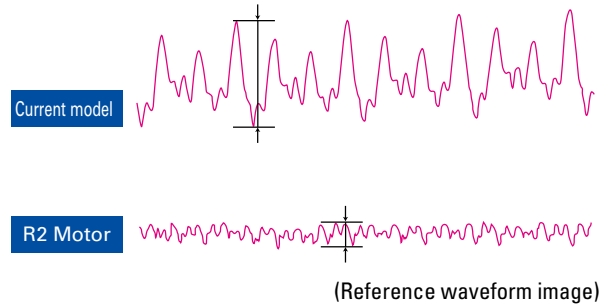
Comparison of cogging torque waveforms
